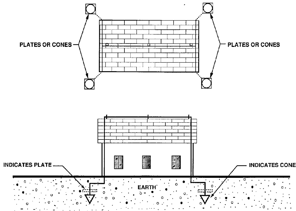
Figure 6-7. Typical buried plates or cones installation
